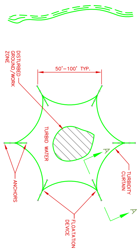
TYPICAL ANCHORING PLAN FOR MID CHANNEL WORK (BRIDGE PIER, CAISSON, ETC.)
